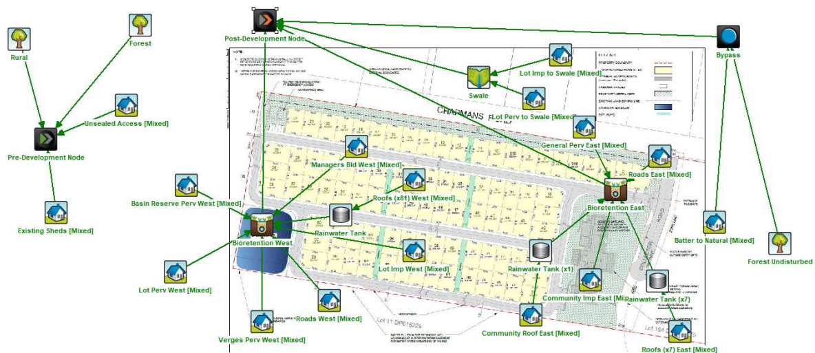
Figure 6-2 MUSIC model layout
