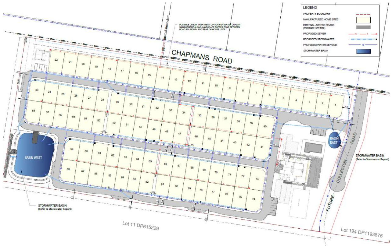
Figure 4-1 Proposed Development Layout
